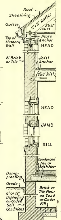
Wall Section
